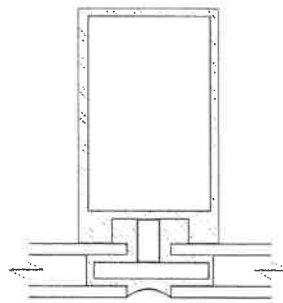
flush glass curtain wall detail
